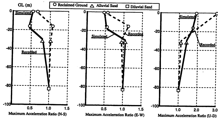
Fig. 17 Distribution of Maximum Acceleration Ratio.
